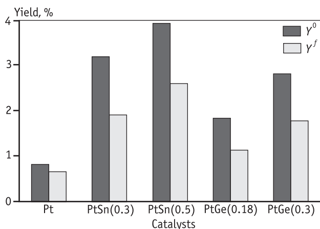
Fig. 12. Initial ( Y^0 ) and final ( Y^f ) yields to 1-decene for Pt, PtSn(0.3 and 0.5 wt.%) and PtGe(0.18 and 0.3 wt.%) supported on \gamma -A/ \alpha -A
