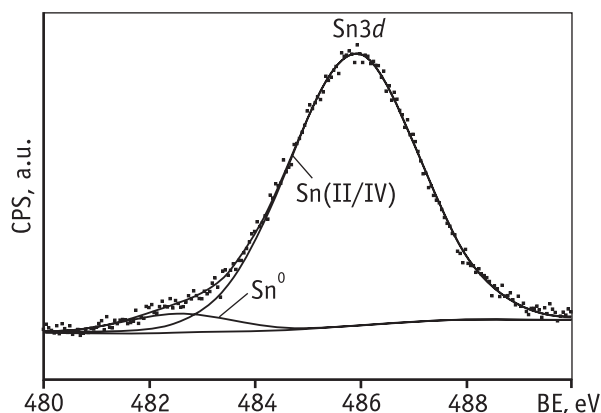
Fig. 6. XPS signals of Sn3d in the PtSn(0.5)/ \gamma -A/ \alpha -A catalyst
