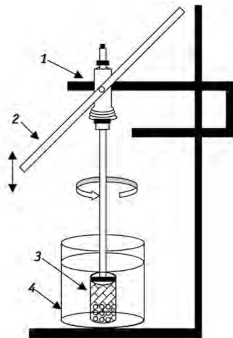
Fig. 1. Diagram of equipment for the deposition of «Coating»:
