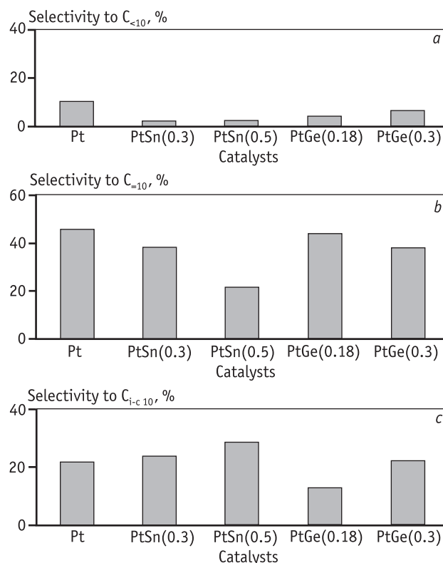
Fig. 13. Mean selectivity values to C_{<10} (a), C_{=10} (b) and C_{i-c10} (c) for Pt, PtSn(0.3 and 0.5 wt.%) and PtGe(0.18 and 0.3 wt.%) supported on \gamma -A/ \alpha -A
