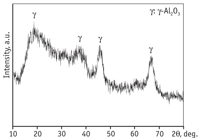
Fig. 3. XRD spectrum of the deposited \gamma - \text{Al}_2\text{O}_3 layers
