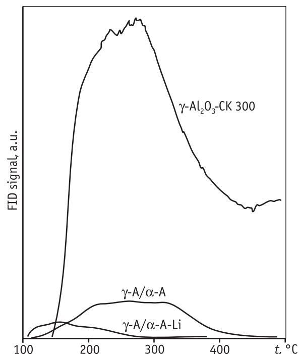
Fig. 4. TPD of pyridine for different samples (layers of \gamma -A, \gamma -A-Li and \gamma - \text{Al}_2\text{O}_3 CK 300)
