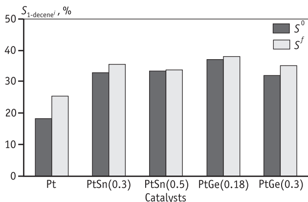
Fig. 11. Initial ( S^0 ) and final ( S^f ) selectivity to 1-decene for the Pt, PtSn(0.3 and 0.5 wt.%) and PtGe(0.18 and 0.3 wt.%) supported on \gamma -A/ \alpha -A
