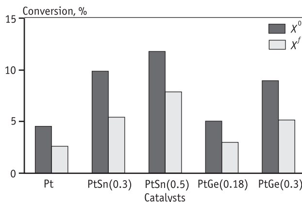
Fig. 8. Initial and final n -decane conversion for Pt/ \gamma -A/ \alpha -A, PtSn(0.3 and 0.5 wt.%) / \gamma -A/ \alpha -A and PtGe(0.18 and 0.3 wt.%) / \gamma -A/ \alpha -A
