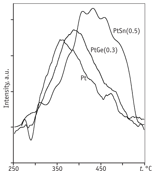
Fig. 10. TPO profiles for catalysts Pt, PtSn and PtGe supported on \gamma -A/ \alpha -A measured at the end of the reaction
